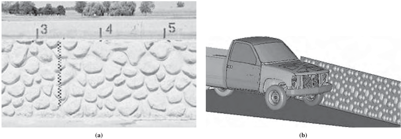
Figure 51. Cobblestone barrier: (a) actual; (b) simulation model.
