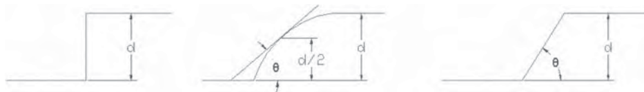
Figure 56. Generalized types of surface asperities.
