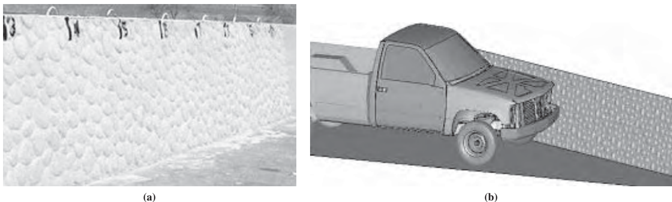
Figure 52. Shallow cobblestone barrier: (a) actual; (b) simulation model.
