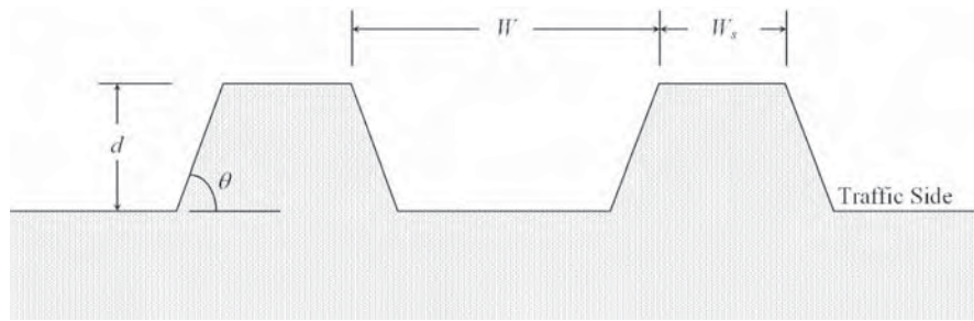
Figure 57. Surface asperity geometry variables.
